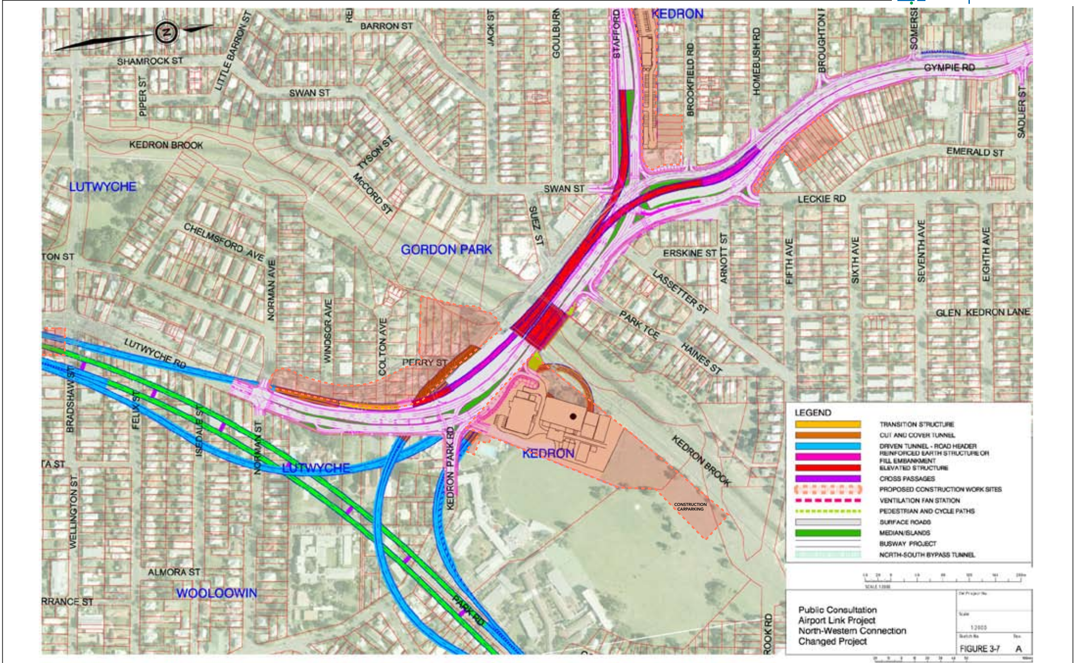
North Western Connection Changed Project Surface Works and Elevated Structure
